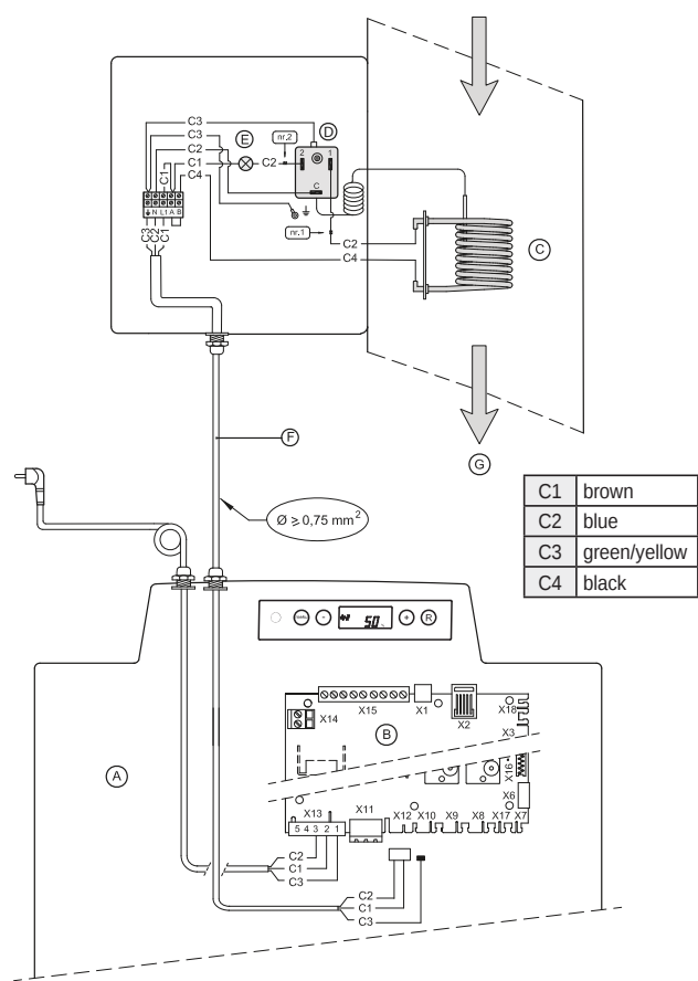
Preheater
